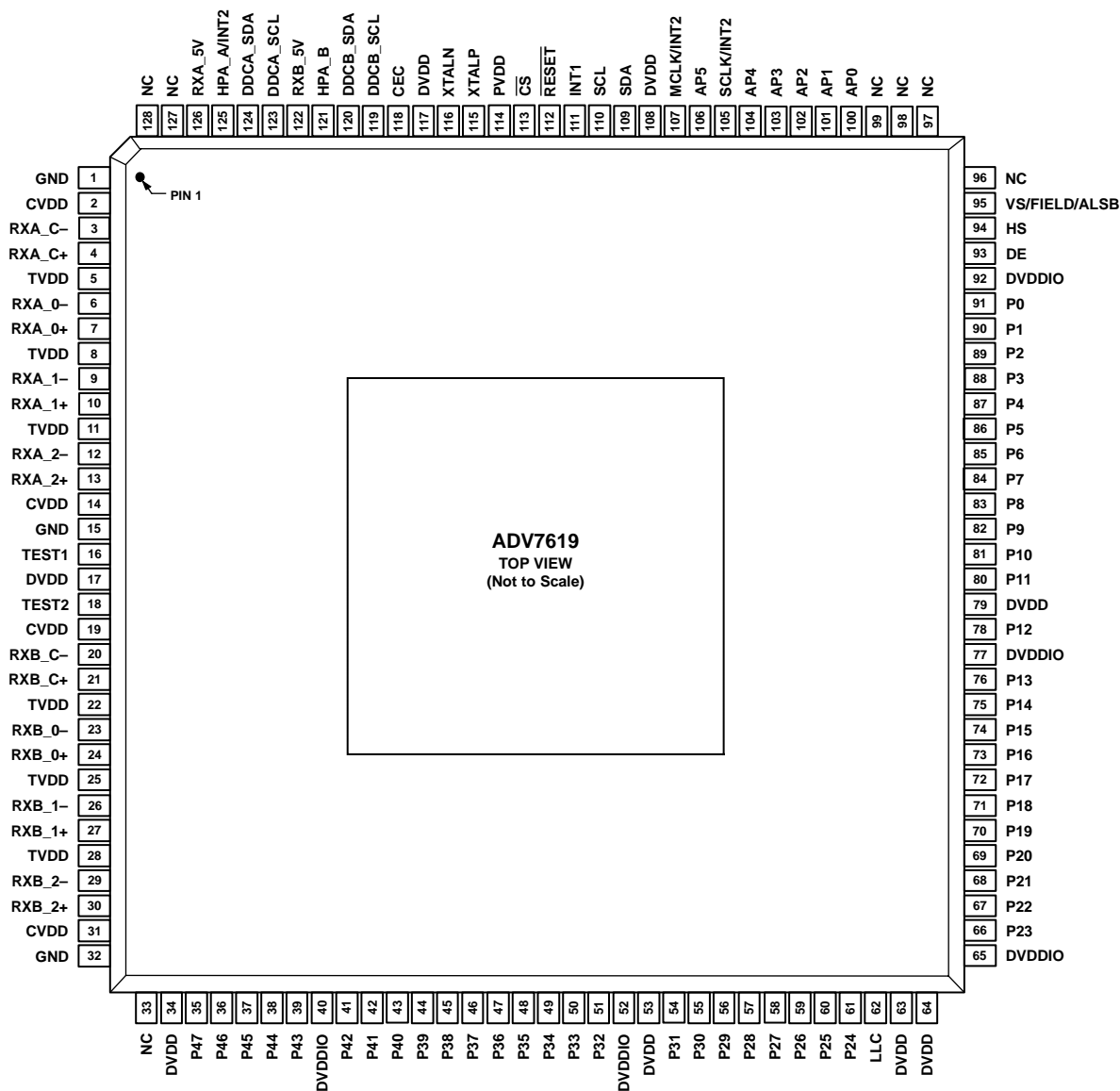
Figure 6. Pin Configuration
