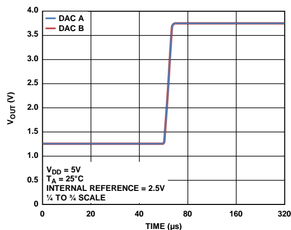
Figure 29. Settling Time
