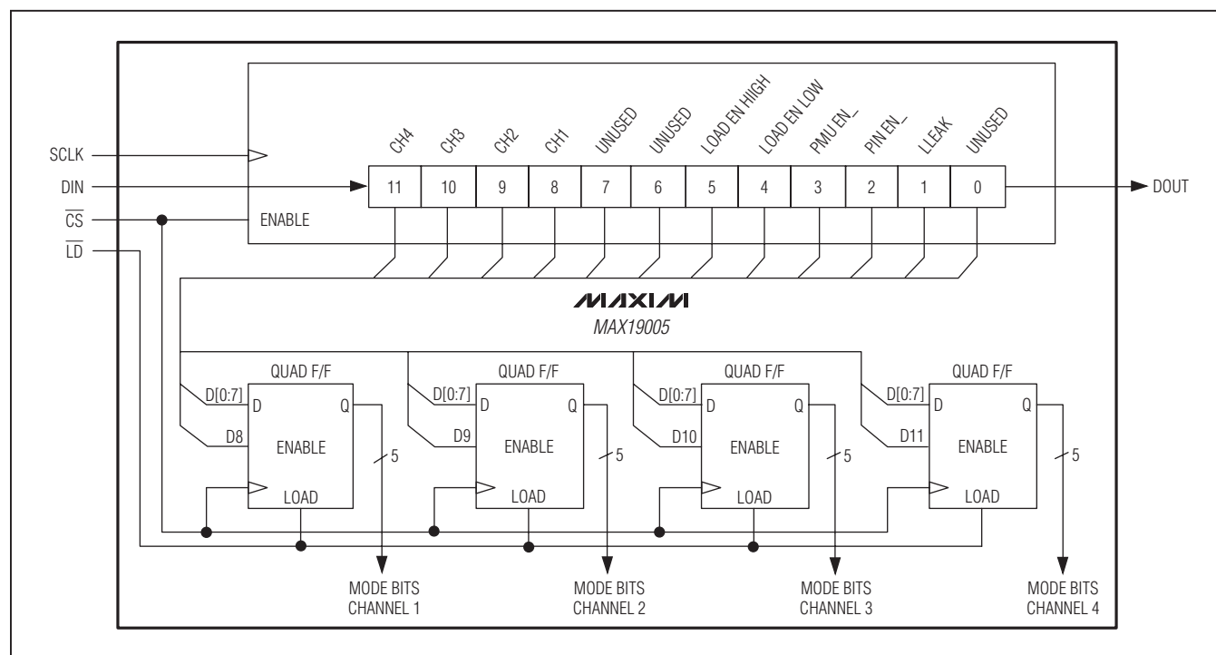
Figure 5. Serial Interface
