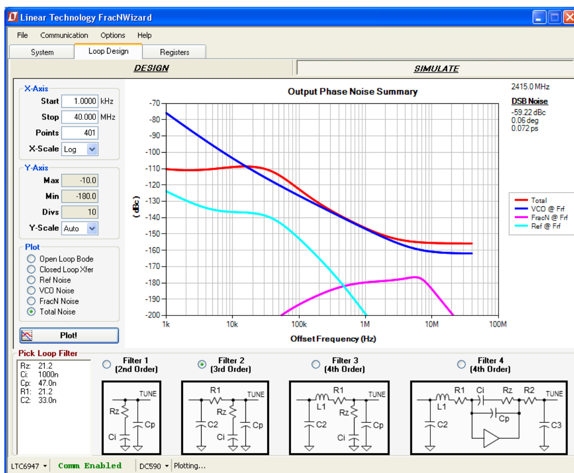
Figure 3. FracNWizard Screenshot
