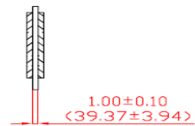
VIEW D-D
