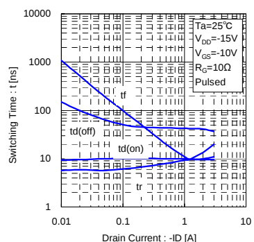
Fig.9 Switching Characteristics
