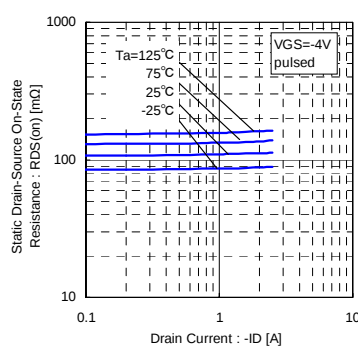
Fig.7 Static Drain-Source On-State Resistance vs. Drain Current
