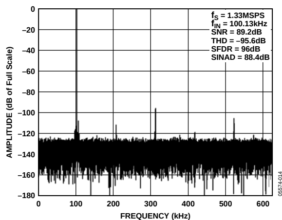
Figure 14. FFT 100 kHz
