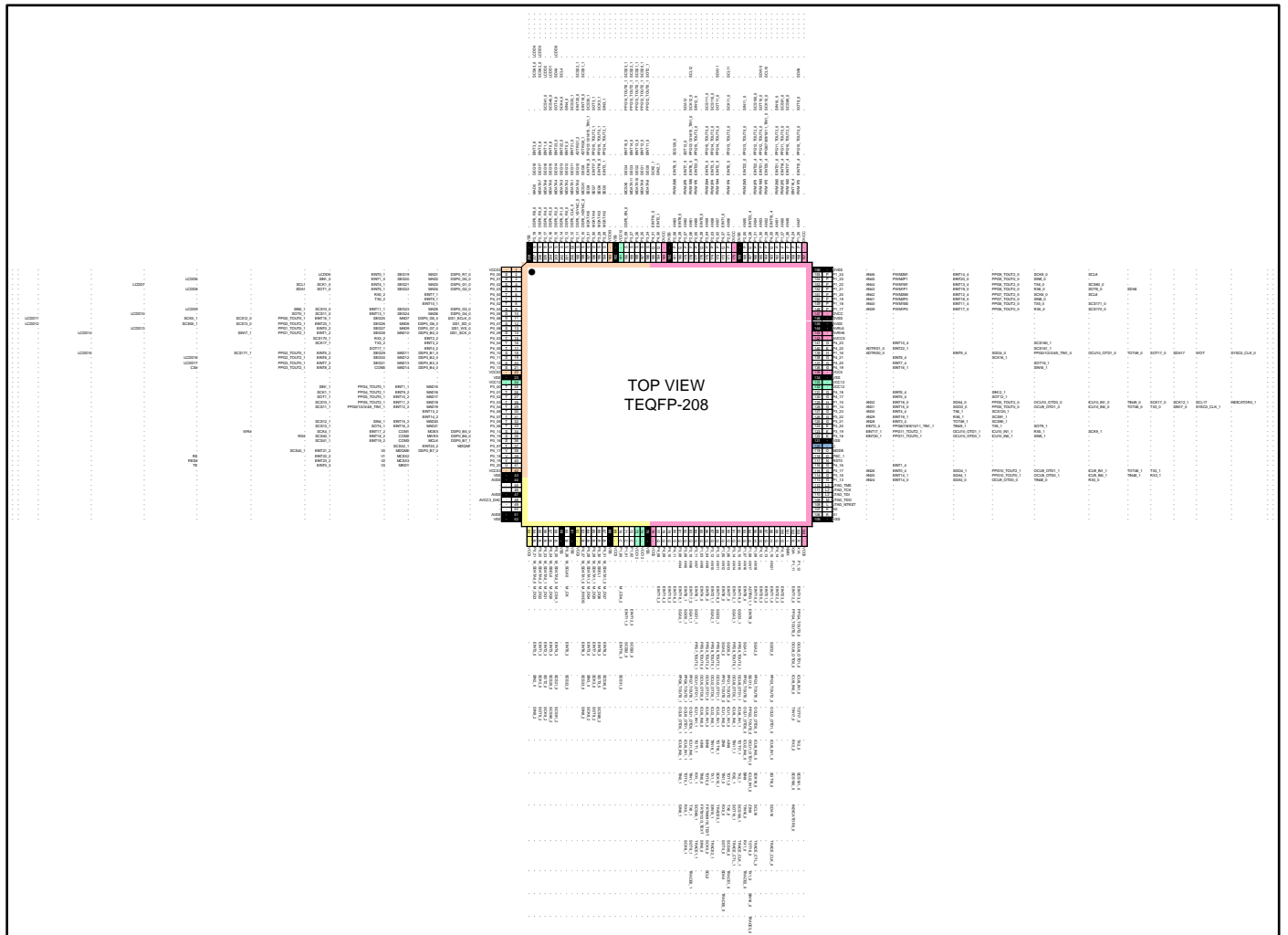
Figure 4-4: TEQFP-208 (S6J334xKyz *1)
