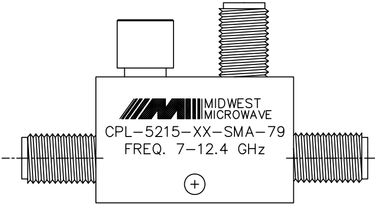
BACKSIDE MARKING
