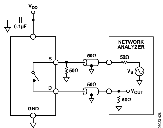
Figure 26. Off Isolation
