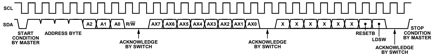
Figure 31. Write Operation
