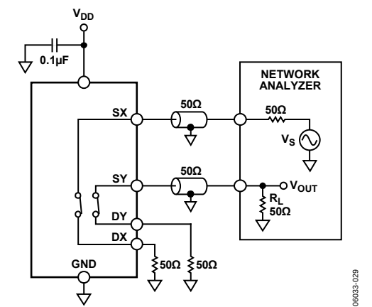
Figure 27. Channel-to-Channel Crosstalk
