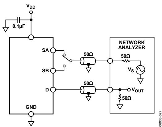
Figure 25. Bandwidth
