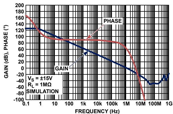
FIGURE 42. OPEN-LOOP GAIN, PHASE vs FREQUENCY, V_S = \pm 15V
