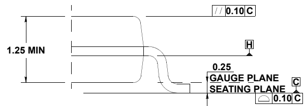
DETAIL "A"
