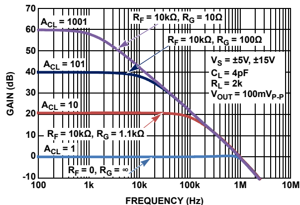
FIGURE 73. CHARACTERIZED CLOSED LOOP GAIN vs FREQUENCY
