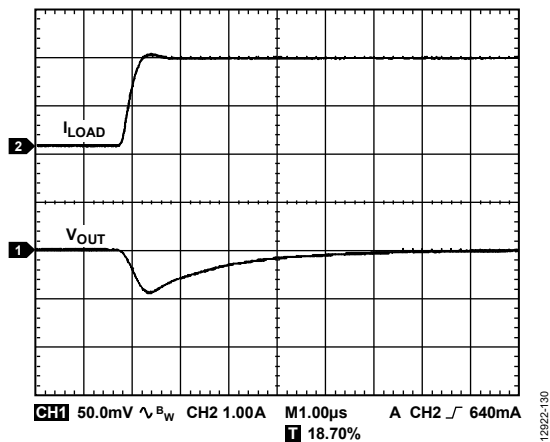
Figure 31. Output Transient Response, C_{\text{OUT}} = 10 \mu\text{F}
