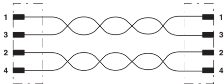
Circuit diagram
