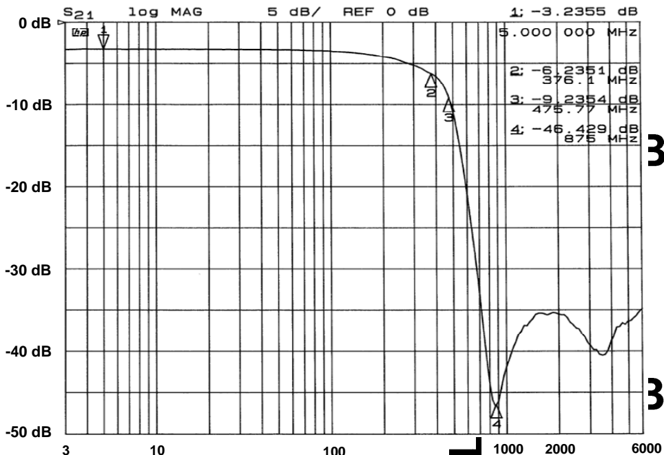
Insertion Loss Vs. Frequency (2.5V Bias)
