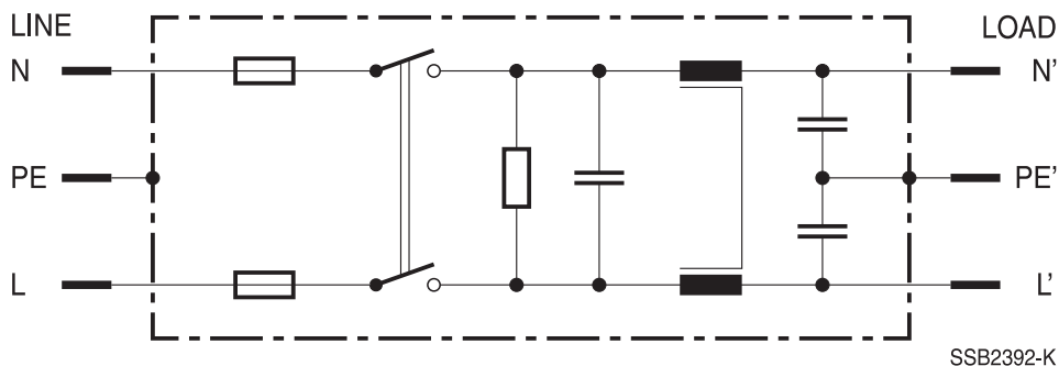
Typical circuit diagram of B84776M* (medical version)
