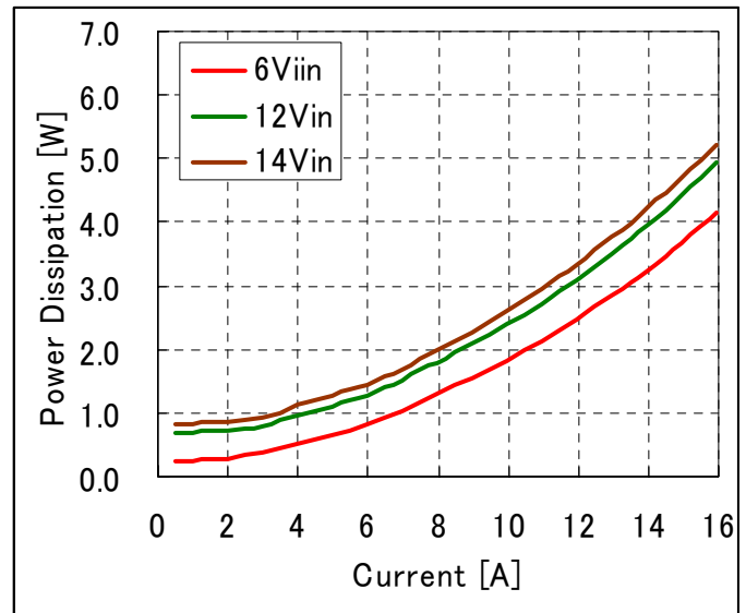
Fig-3.3V-3: Power Loss vs. load current and input voltage for Vout=3.3V. Airflow rate=200 LFM (1m/s) and Ta=25°C.
