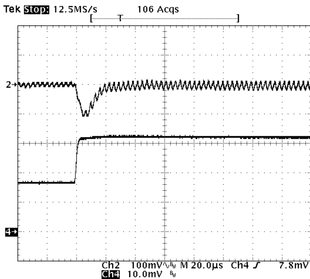
Fig-3.3V-6: Output voltage response for V_{out}=3.3V to positive load current step-change from 8A to 16A with slew rate of 5A/\mu s at V_{in}=12V . C_o=47\mu F \times 4 ceramic. Top trace: output voltage (100mV/div.) Bottom trace: load current (5A/div.) Time scale: 20us/div.
