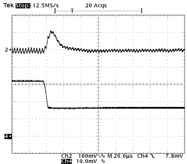
Fig-3.3V-7: Output voltage response for V_{out}=3.3V to negative load current step change from 16A to 8A with slew rate of -5A/\mu s at V_{in}=12V . C_o=47\mu F \times 4 ceramic. Top trace: output voltage (100mV/div.) Bottom trace: load current (5A/div.) Time scale: 20us/div.
