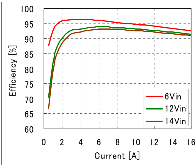
Fig-3.3V-2: Efficiency vs. load current and input voltage for Vout=3.3V. Airflow rate=200 LFM (1m/s) and Ta=25°C.
