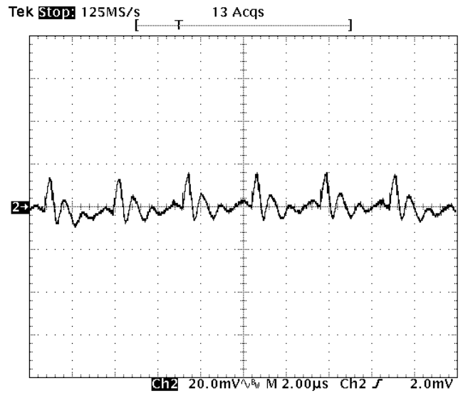
Fig-1.0V-5: Output voltage ripple (20mV/div.) for V_{out}=1.0V at full rated load current into a resistive load with external capacitance 47uFx4 ceramic + 1uF ceramic at V_{in}=12V . Time scale: 2 us/div
