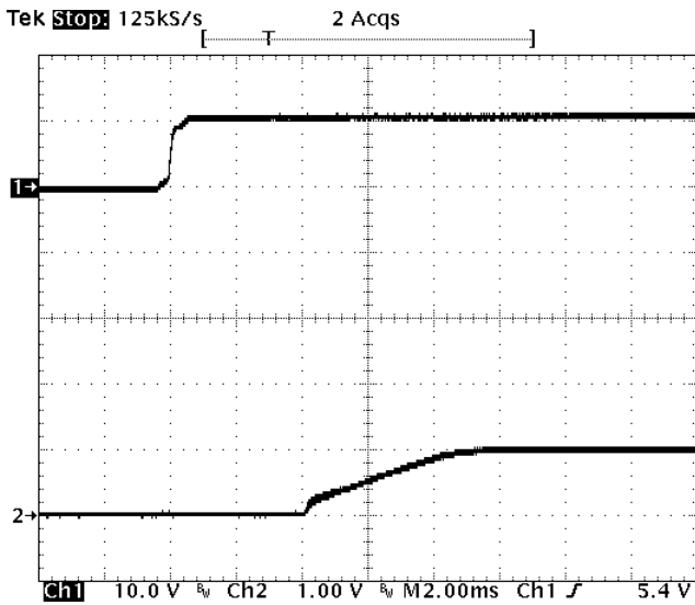
Fig-1.0V-4: Turn-on transient for V_{out}=1.0V with application of V_{in} at full rated load current (resistive) and 47uFx4 external capacitance at V_{in}=12V . Top trace: V_{in} (10V/div.) Bottom trace: output voltage (1V/div.) Time scale: 2 ms/div.
