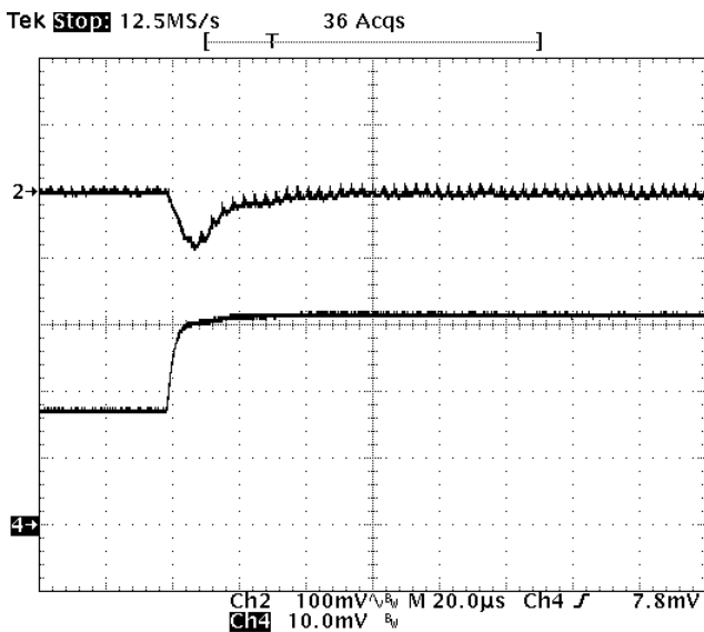
Fig-1.0V-6: Output voltage response for V_{out}=1.0V to positive load current step change from 8A to 16A with slew rate of 5A/us at V_{in}=12V . C_o=47uFx4 ceramic. Top trace: output voltage (100mV/div.) Bottom trace: load current (5A/div.) Time scale: 20us/div.
