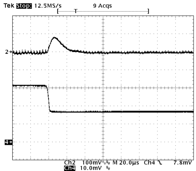
Fig-1.0V-7: Output voltage response for V_{out}=1.0V to negative load current step change from 16A to 8A with slew rate of -5A/us at V_{in}=12V . C_o=47uFx4 ceramic. Top trace: output voltage (100mV/div.) Bottom trace: load current (5A/div.) Time scale: 20us/div.
