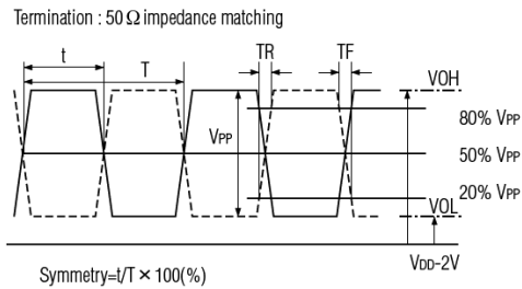
Figure 5) Output Waveform (1)
