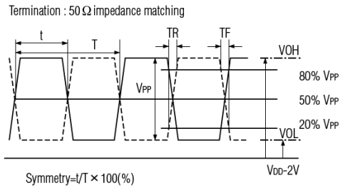
Figure 6) Output Waveform (2)
