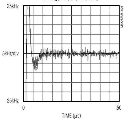
TX-RX TURNAROUND FREQUENCY SETTLING
