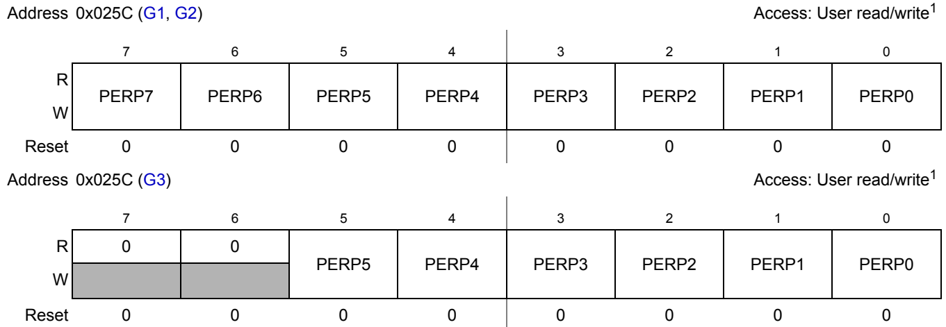
Figure 2-38. Port P Pull Device Enable Register (PERP)
