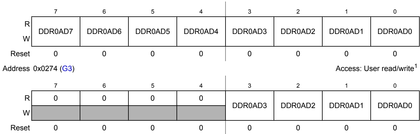
Figure 2-53. Port AD Data Direction Register (DDR0AD)
