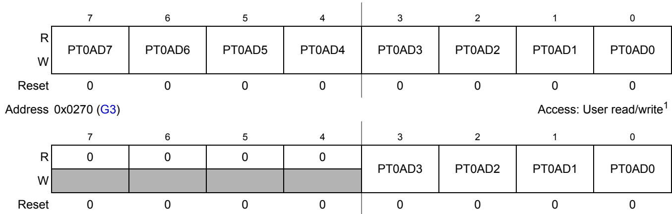
Figure 2-49. Port AD Data Register (PT0AD)
