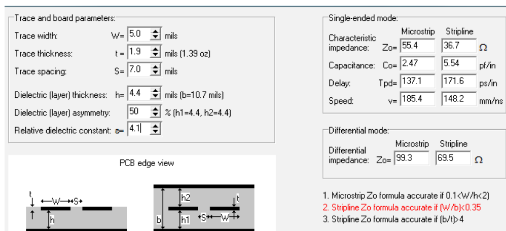
Figure 7-10 Trace Width and Clearance of Micro-strip and Strip-line
