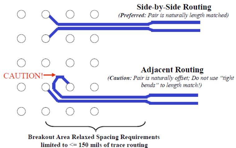
Figure 7-14 Layout Guidance of Matched Differential Pair
