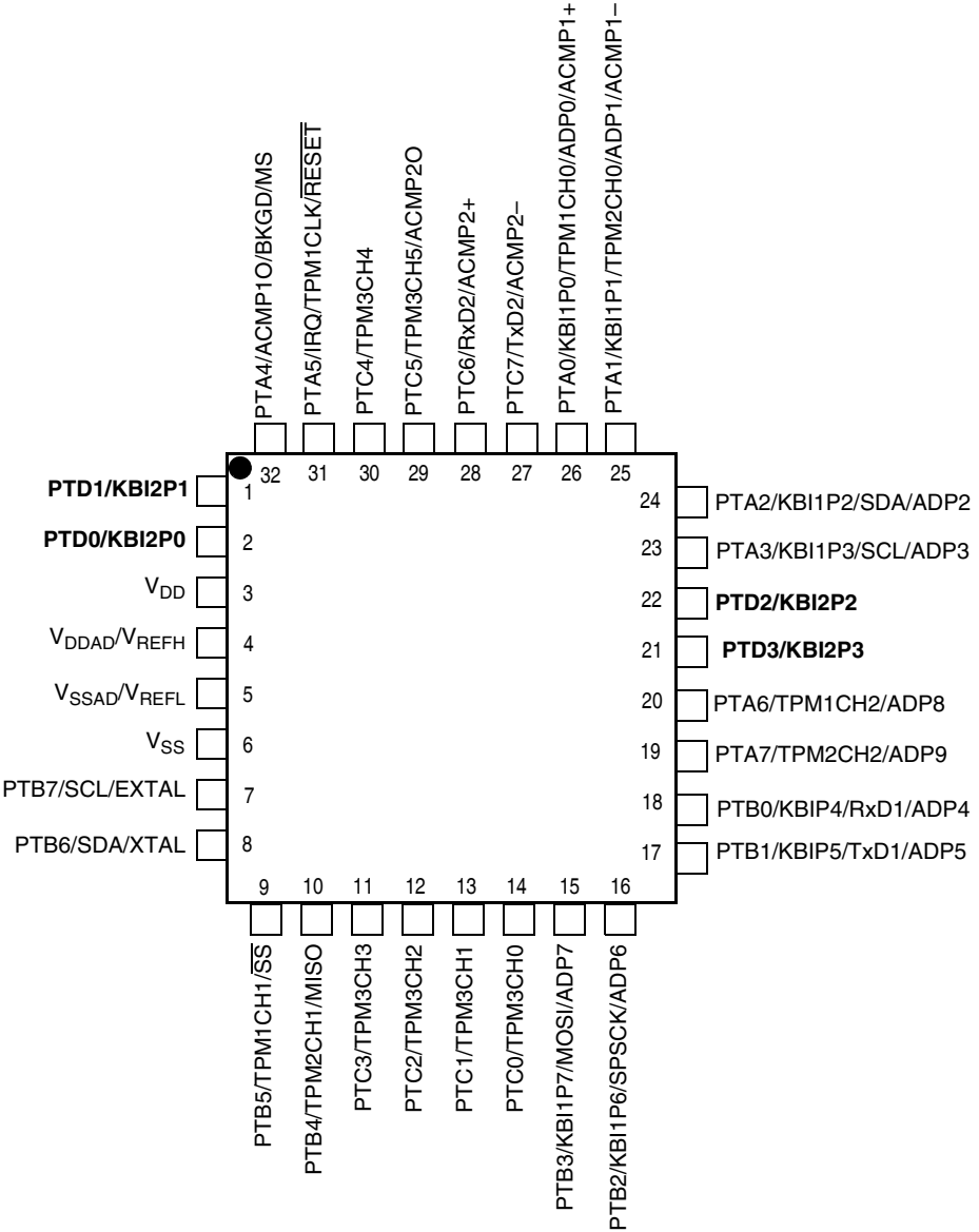
Figure 4. 32-Pin LQFP/QFN
