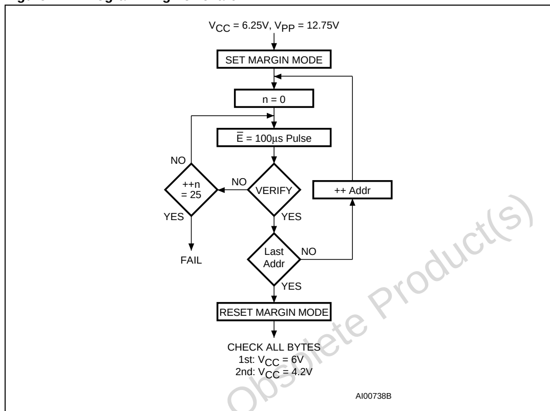
Figure 4. Programming flowchart
