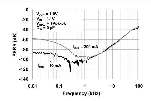
FIGURE 2-24: Power Supply Ripple Rejection vs. Frequency.
