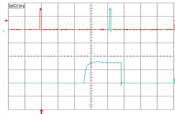
Figure 14. Load current (top trace, 20 A/div., 50 ms/div.) into a 10 m short circuit during restart, at V_{in} = 48 V. Bottom trace (20 A/div., 2 ms/div.) is an expansion of the on-time portion of the top trace
