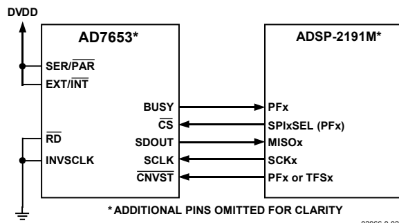
Figure 37. Interfacing the AD7653 to an SPI Interface
