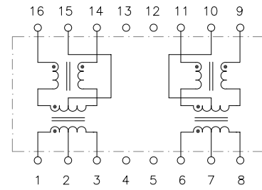
Circuit D
