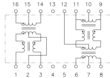
N6 Package
