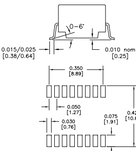
Recommended Solder Pad Dimensions
