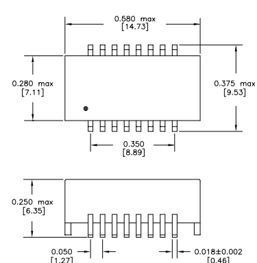
N6 Package
