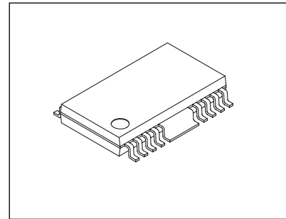
HSSOP16(275mil)
