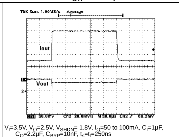
Figure 28. Load transient ( C_O = 2.2 \mu\text{F} , C_{BYP} = 10 \text{ nF} )
