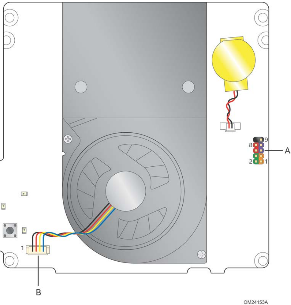
Figure 12. Headers and Connectors (Top)
