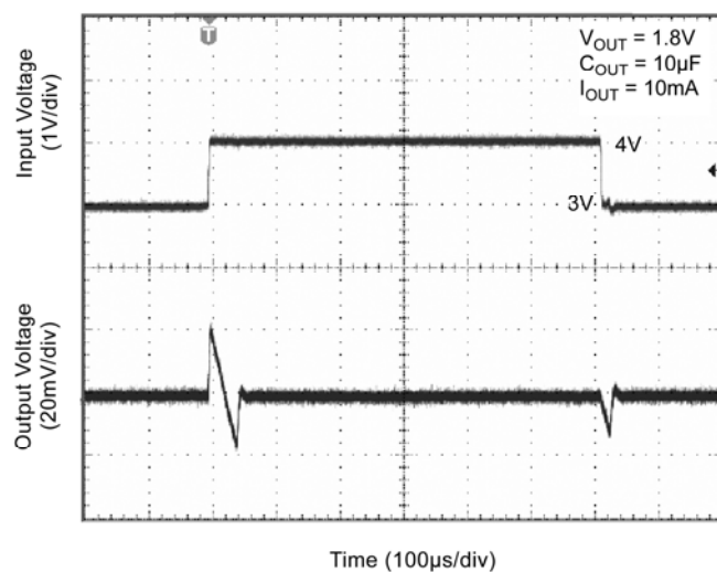
Line Transient
