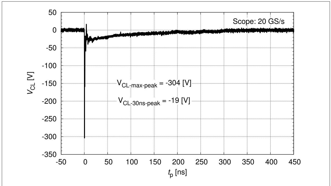
Figure 6 Clamping voltage (ESD): V_{CL} = f(t) , 8 kV negative pulse from pin 1 to pin 2
