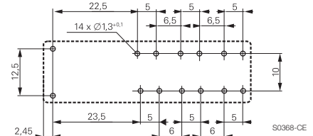
5 form A + 1 form B, 5 NO + 1 NC versions SR6 C
