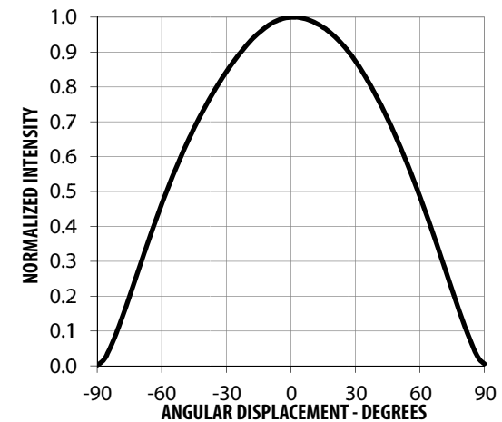
Figure 12 Radiation Pattern
