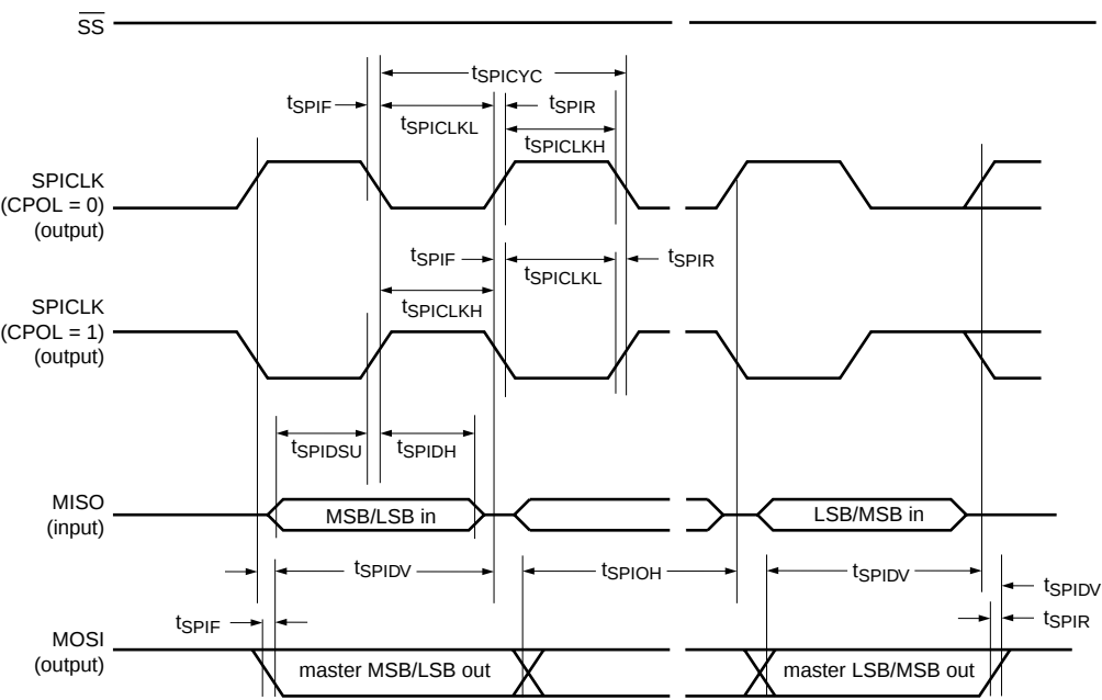
Fig 25. SPI master timing (CPHA = '1').
