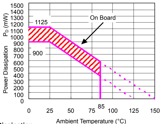
Power Dissipation
