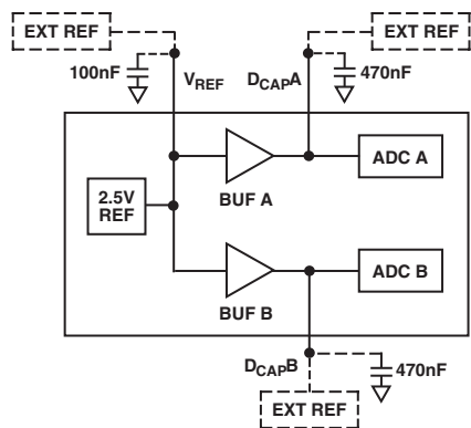
Figure 15. Reference Circuit
