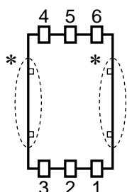
SON-6 Pin Configuration
