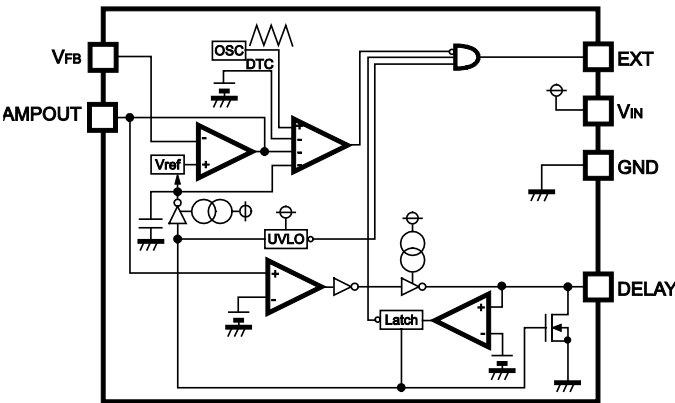
R1211x002A/C Block Diagram
