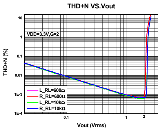
THD+N vs. V_{\text{OUT}}
