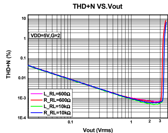
THD+N vs. V_{\text{OUT}}
