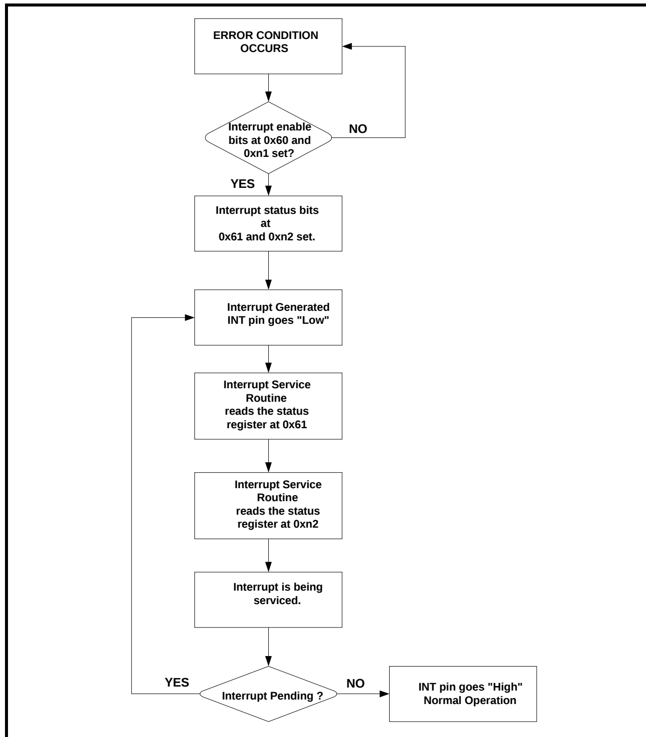
FIGURE 38. INTERRUPT PROCESS
