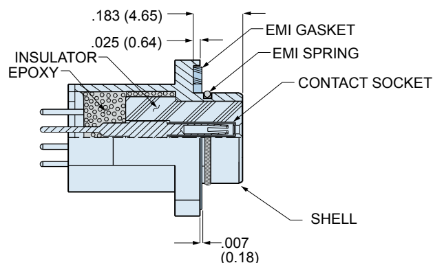
CROSS-SECTIONAL VIEW OF 790-029S
