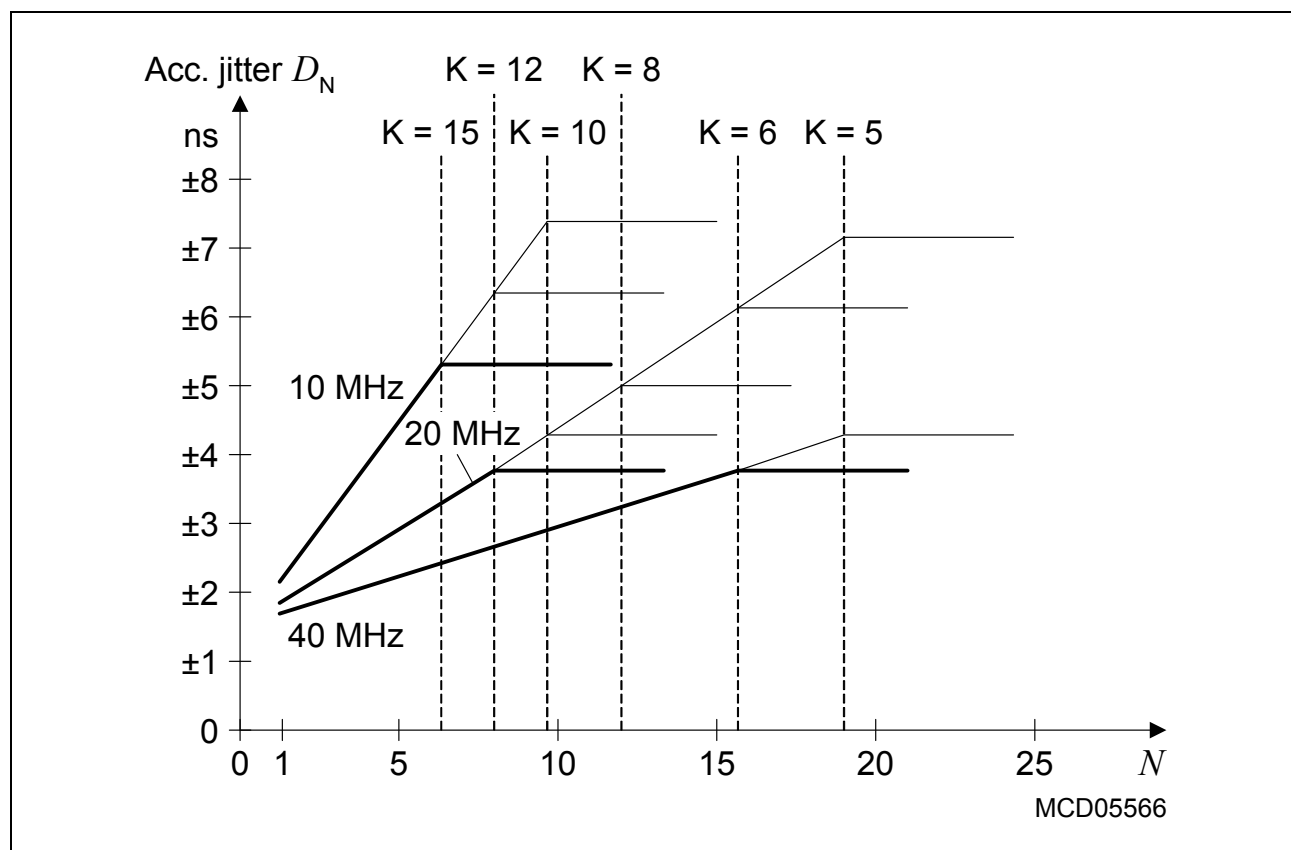
Figure 16 Approximated Accumulated PLL Jitter
