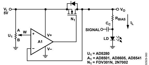
Figure 60. Programmable Booster Voltage Source
