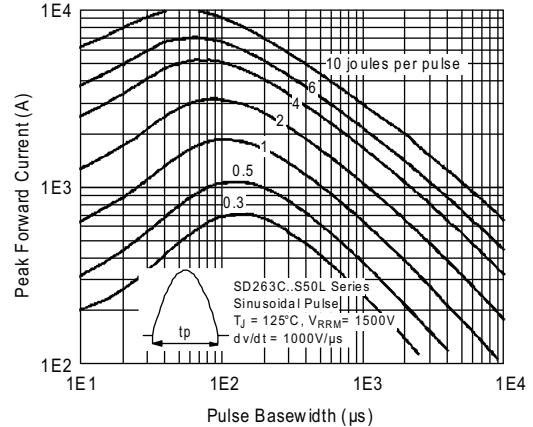
Fig. 15 - Maximum Total Energy Loss Per Pulse Characteristics
