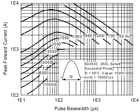
Fig. 16 - Frequency Characteristics
