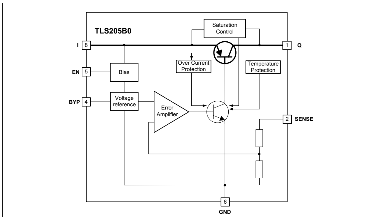
Figure 1 Block Diagram TLS205B0 V50
