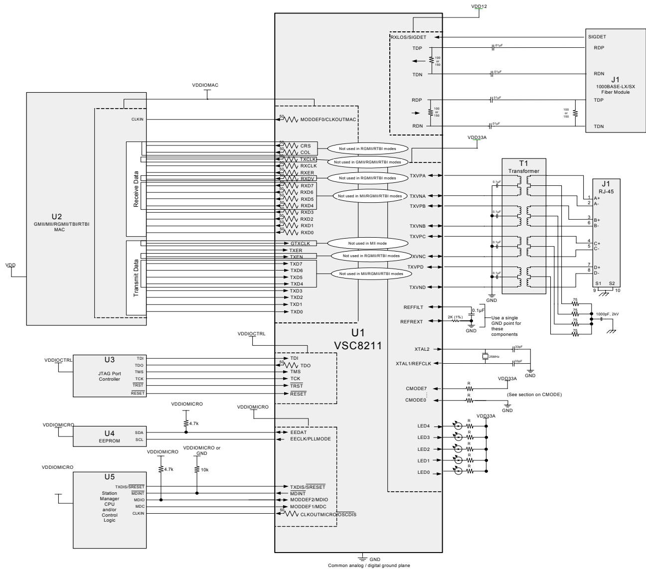
Figure 10. System Schematic – ‘Parallel Data MAC to Copper/Fiber Auto Media Sense’ PHY Operating Mode
